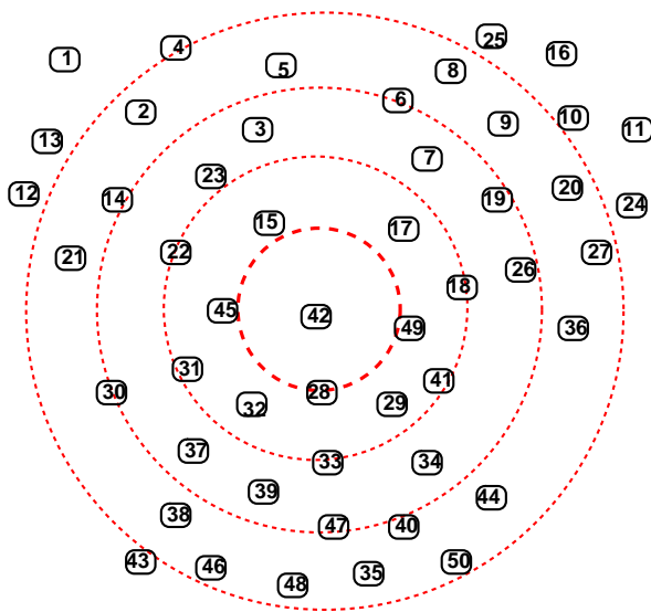
Figure 4.1: Dissemination of routing information in ad hoc wireless networks. The sequence of dotted circles from small to big indicates the propagation of routing information from the source node 42 through whole networks. Node 42 is the center of all dotted circles and the process is like a ripple.
