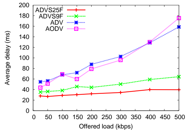
Figure 5.25: Average delays (offerloads from 0 to 500 kbps) achieved for CBR traffic on 1000-node ad hoc networks.
